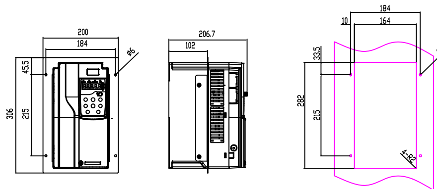
Flange Mounting
