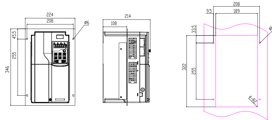
Flange Mounting
